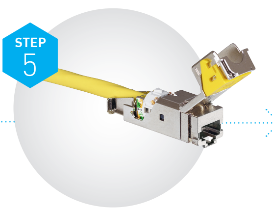
Install the wire housing without pushing
